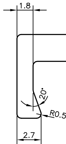
DETAIL OF 'A' SCALE 4:1
