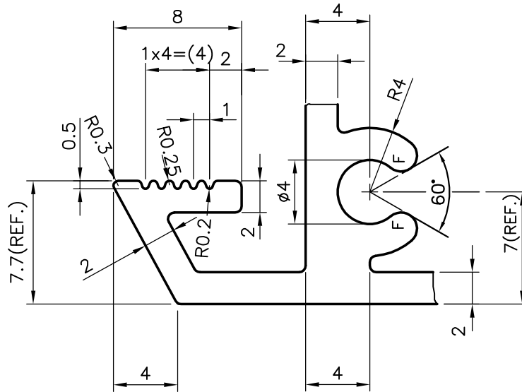
DETAIL OF "A" SCALE 3:1
