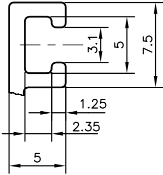
DETAIL OF "A" SCALE:- 3:1
