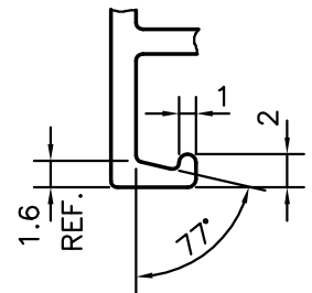
DETAILS OF "B" SCALE 2:1
