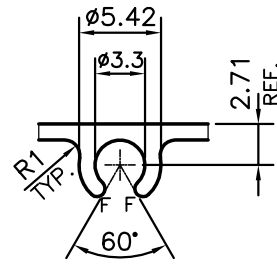
DETAIL OF "B" SCALE:- 2:1
