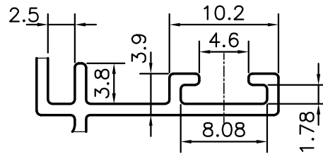
DETAIL OF "B" SCALE:- 2:1
