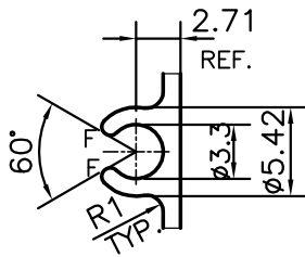
DETAIL OF "A" SCALE:- 2:1
