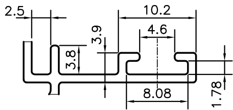
DETAIL OF "B" SCALE:- 2:1
