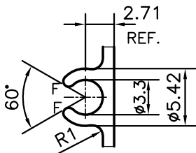
DETAIL OF "A" SCALE:- 2:1
