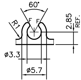
DETAIL OF "B" SCALE:- 2:1
