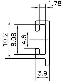
DETAIL OF "A" SCALE:- 2:1
