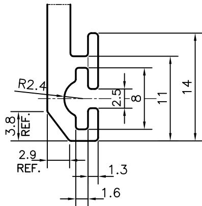
DETAIL OF "A" SCALE 2:1
