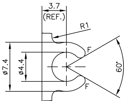
DETAILS OF "A" SCALE 3:1
