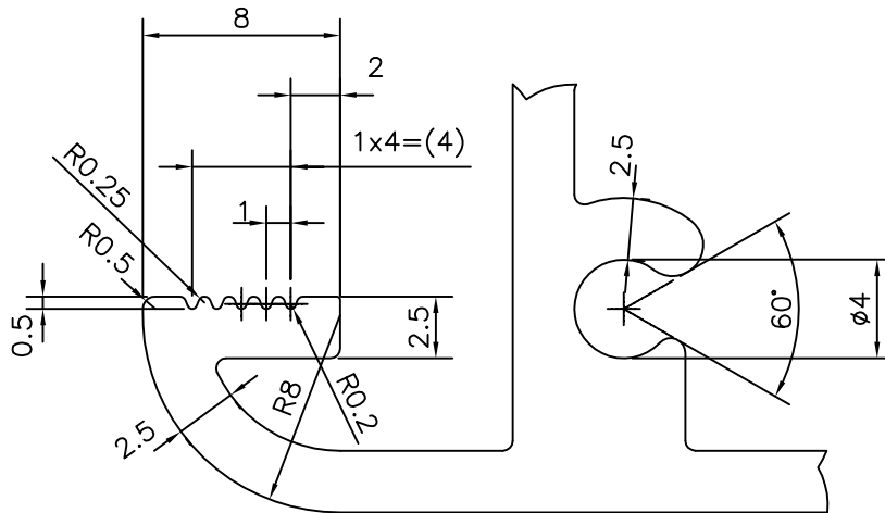
DETAIL OF "A" SCALE 3:1
