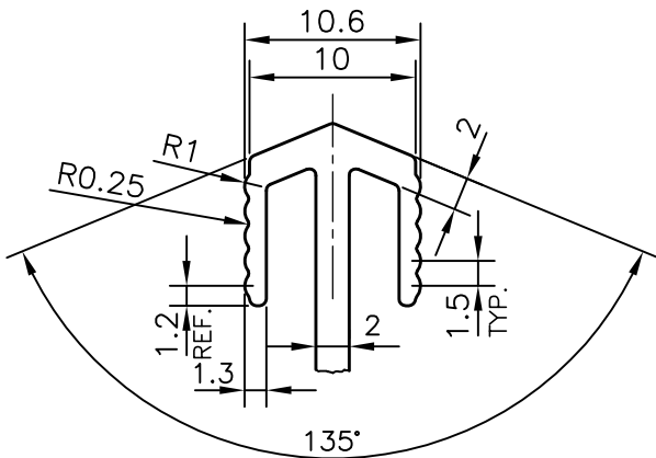
DETAIL OF "A" "B" SCALE 2:1
