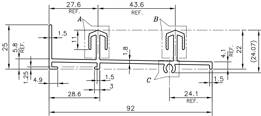
DETAIL OF "C" SCALE 2:1
