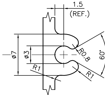
DETAILS OF "A" SCALE 3:1
