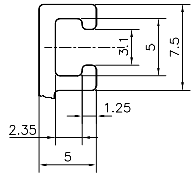
DETAIL OF "C" SCALE 3:1
