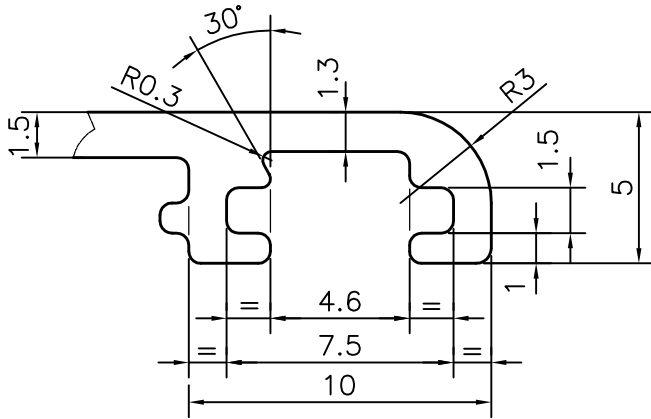
DETAIL OF "A" SCALE 4:1
