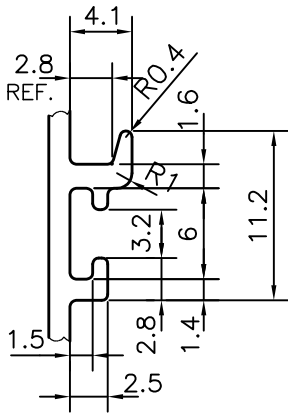
DETAIL OF "B" SCALE 2:1
