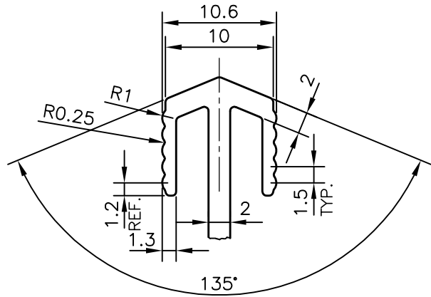
DETAIL OF "A" SCALE 2:1
