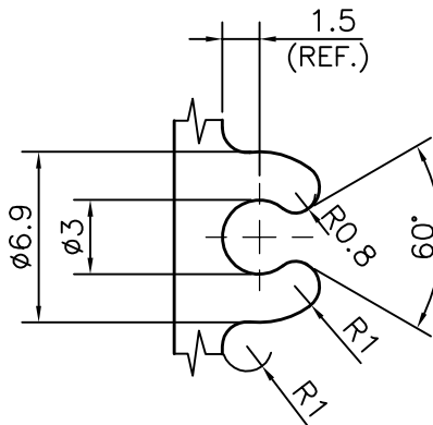
DETAILS OF "A" SCALE 3:1
