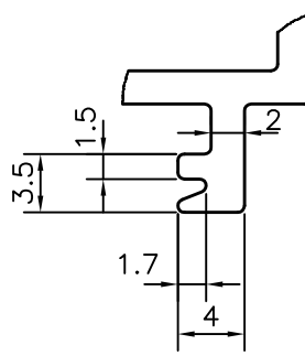
DETAIL OF "B" SCALE 2:1
