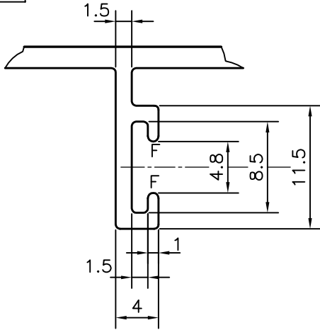
DETAIL OF "A" SCALE 2:1
