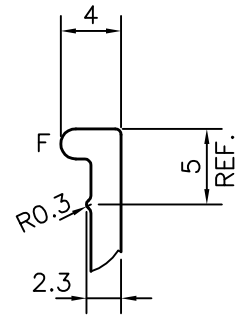
DETAIL OF "C" SCALE 2:1
