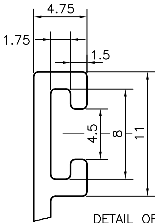
DETAIL OF "A" SCALE 3:1
