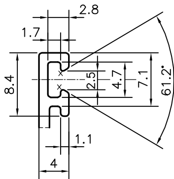
DETAIL OF "A" SCALE 2:1
