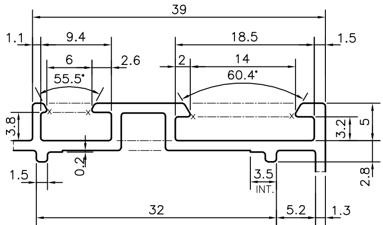
DETAIL OF "B" SCALE 2:1
