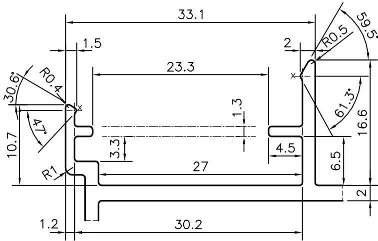
DETAIL OF "C" SCALE 2:1
