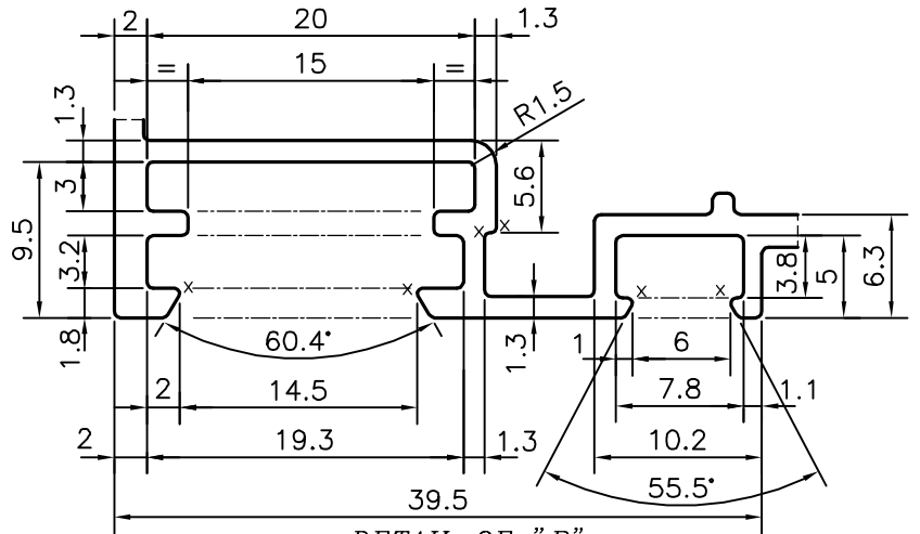
DETAIL OF "B" SCALE 2:1
