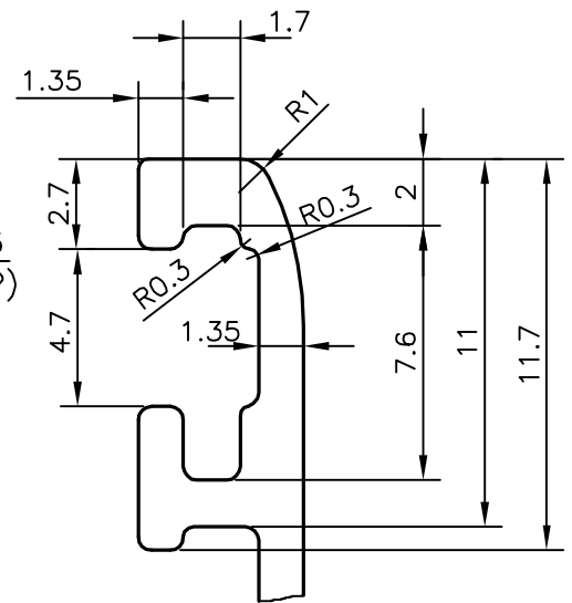
DETAILS OF "A" SCALE 4:1
