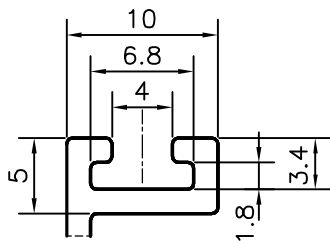
DETAIL OF "A" SCALE 2:1
