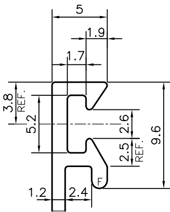
DETAIL OF "A" SCALE :- 3:1
