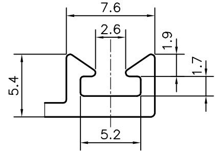
DETAIL OF "B" SCALE- 3:1
