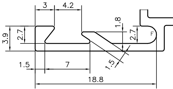
DETAIL OF "A" SCALE- 3:1
