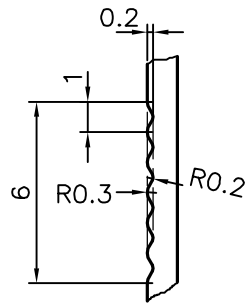
DETAIL "B" SCALE 4:1
