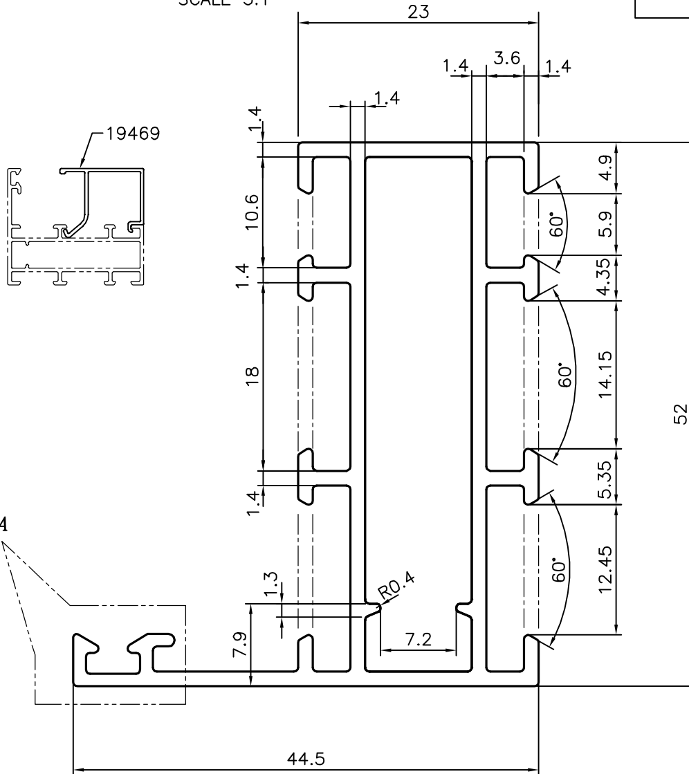
DETAIL OF "A" SCALE 3:1
