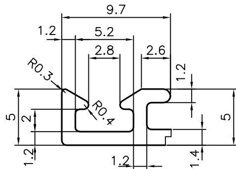
DETAIL OF "A" SCALE 3:1
