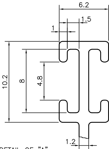
DETAIL OF "A" SCALE 4:1
