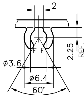
DETAIL OF "B" SCALE 2:1
