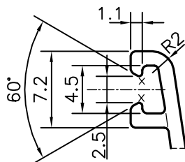
DETAIL OF "A" SCALE 2:1
