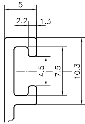
DETAIL OF "A" SCALE 3:1
