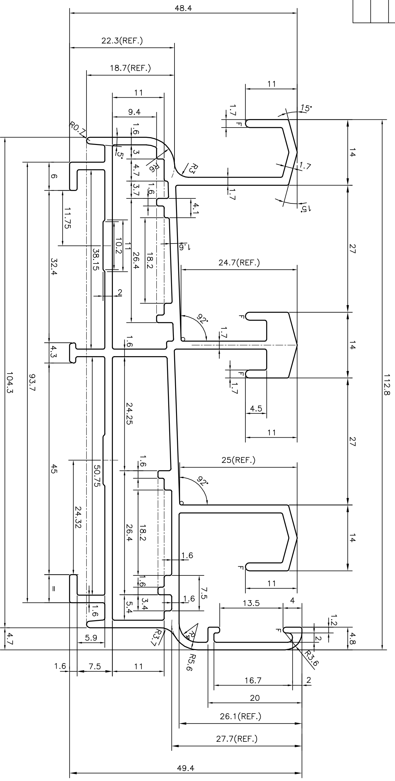
ASSEMBLY SECTION :- S4929,S4930
