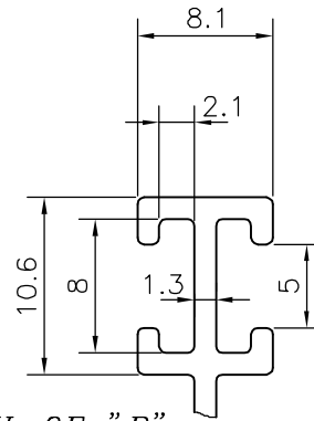
DETAIL OF "B" SCALE 2:1
