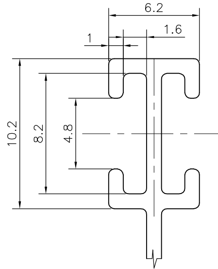
DETAILS OF "A" SCALE 4:1
