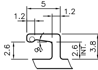
DETAIL OF "A" SCALE 3:1
