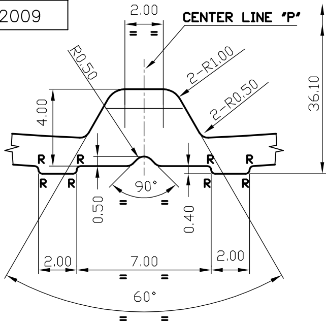
DETAILS "A" SCALE = 5:1 R = RADII 0.20 (8)
