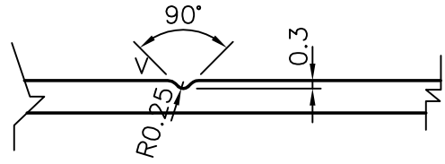
DETAIL V GROOVE
