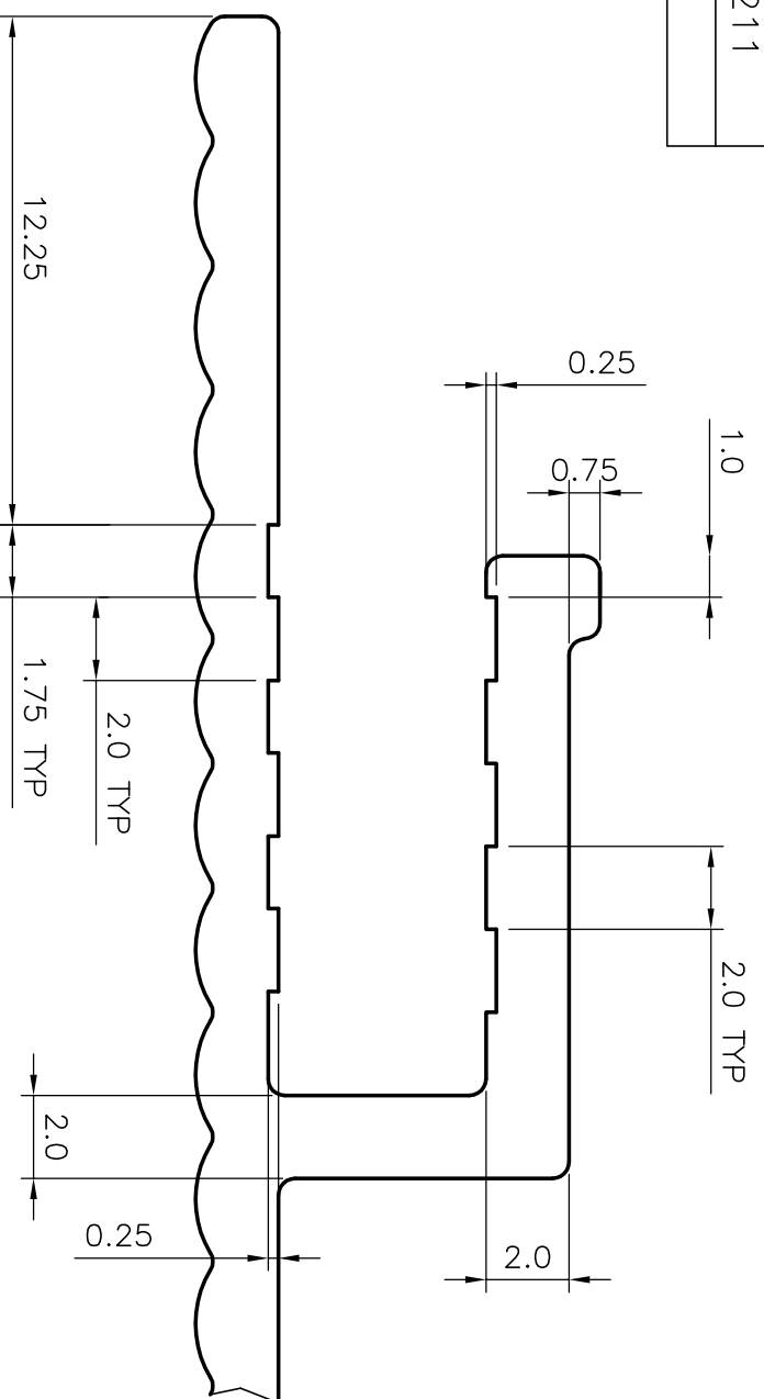
DETAIL A SCALE 5:1
