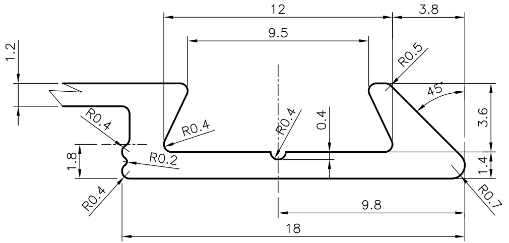
DETAIL "B" SCALE 5:1
