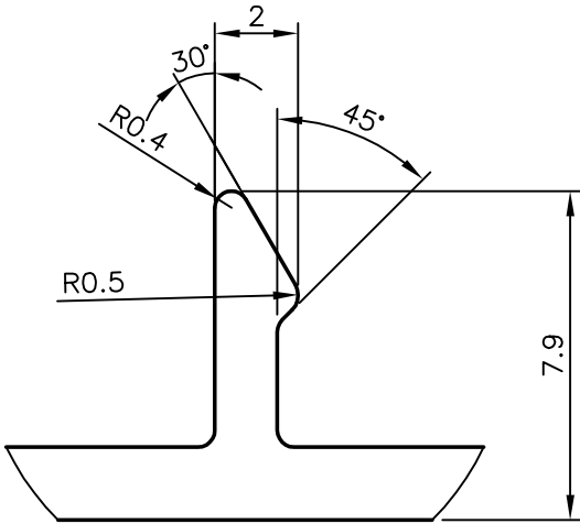
DETAIL OF "A" SCALE 5:1
