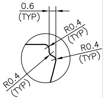
DETAIL OF "A" SCALE 5:1
