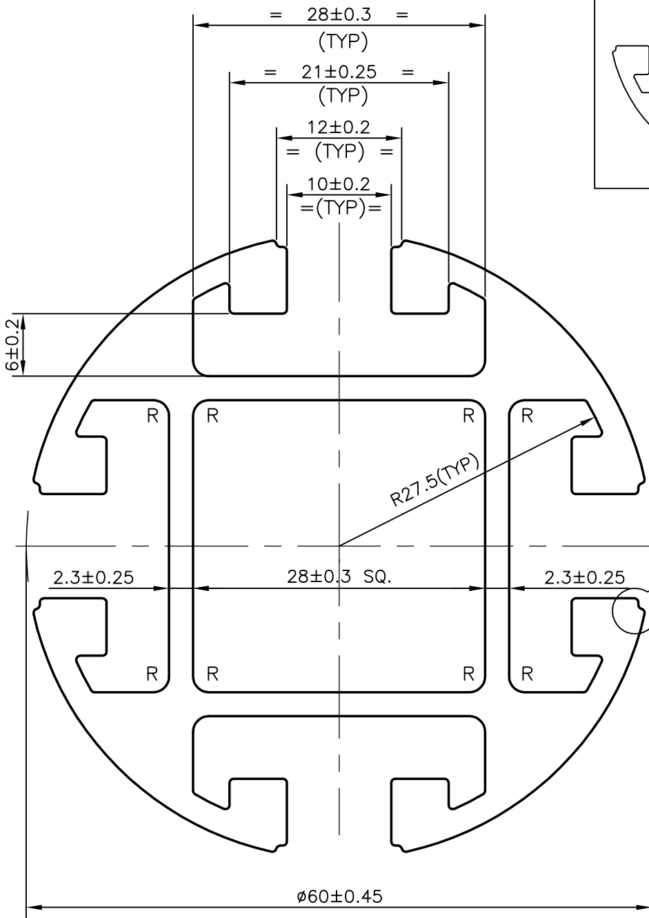
DETAIL OF "A" SCALE 5:1
