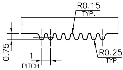
DETAIL OF "A" SCALE 4:1
