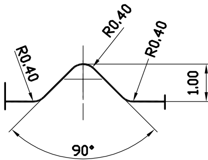
DETAILS "A" SCALE 10:1
