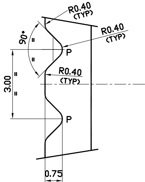
DETAILS "B" SCALE 10:1
