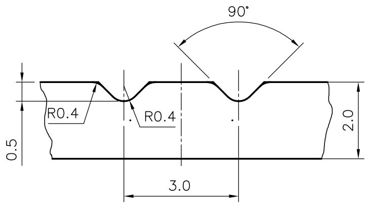
SCALE 10:1 DETAIL A
