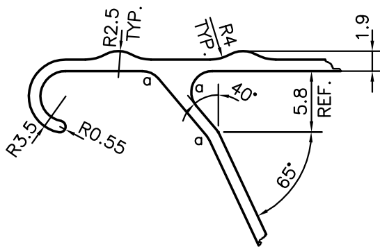
DETAIL OF 'A' SCALE 2:1
