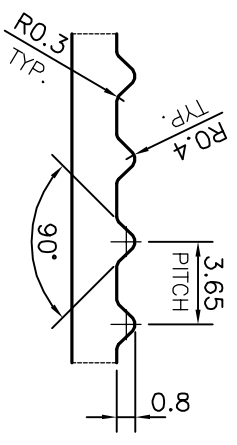
DETAIL OF "A" SCALE 3:1 TYP. DETAIL
