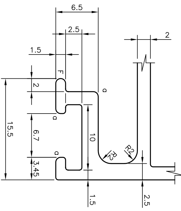
DETAIL OF "B" SCALE 3:1
