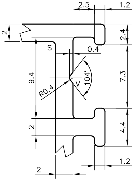
DETAIL "A" SCALE 4:1
